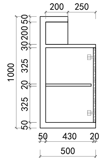
sectional view
