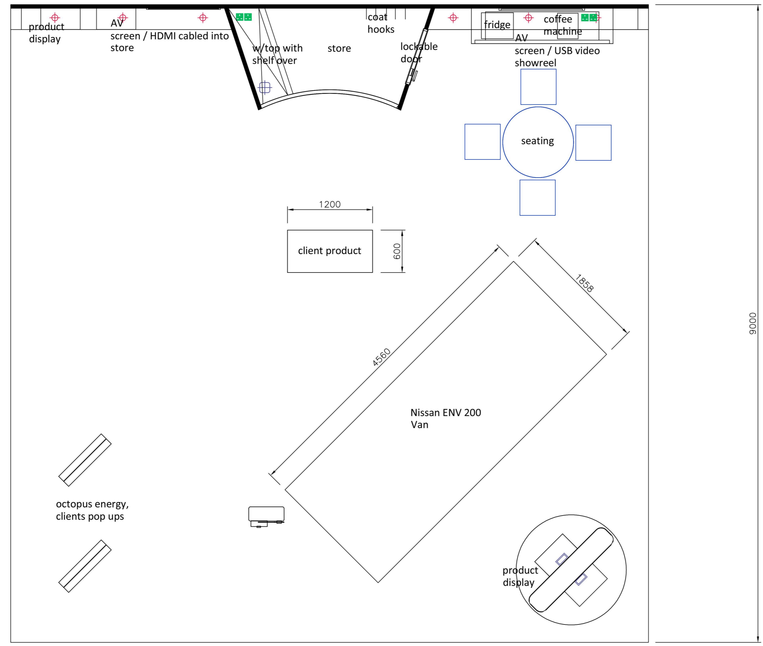
Plan Layout
