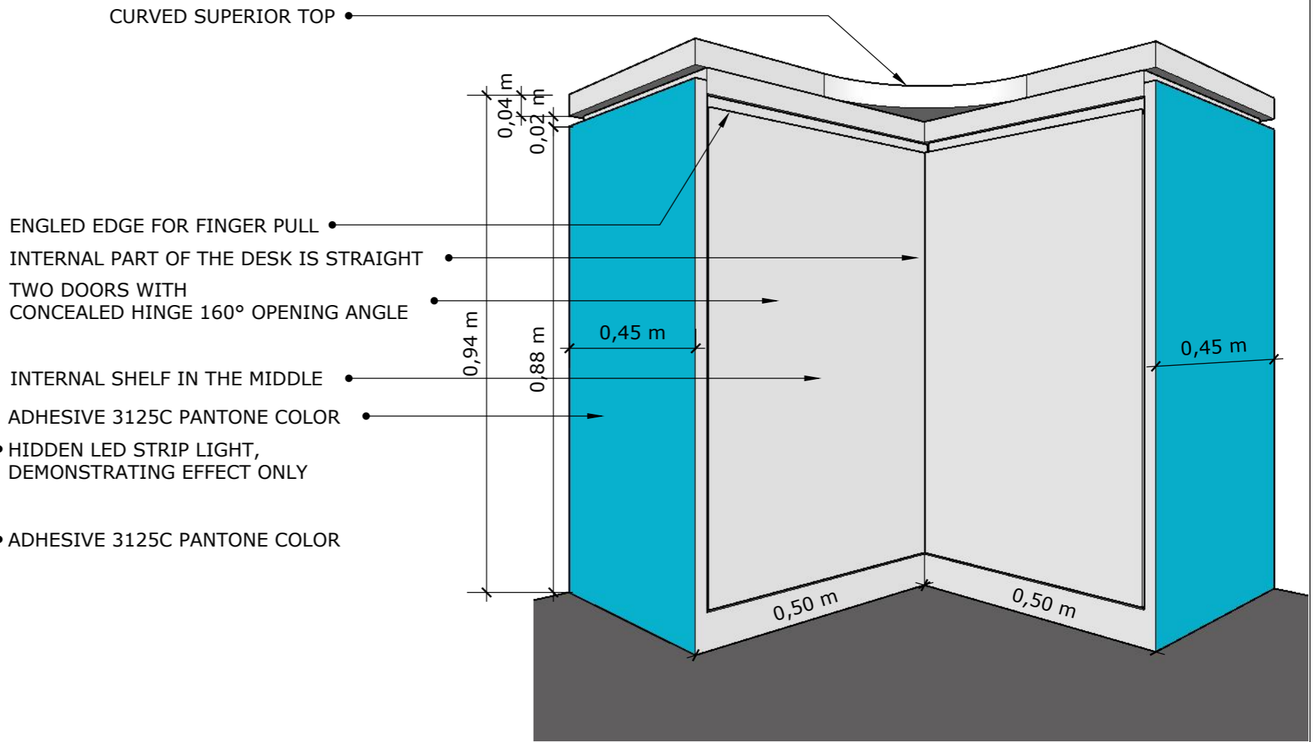
INTERNAL VIEW SERVICE AND SUPPORT DESK - WITHOUT SCALE
