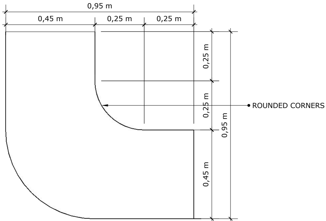
FLOOR PLAN SERVICE AND SUPPORT DESK - SCALE 1/10
