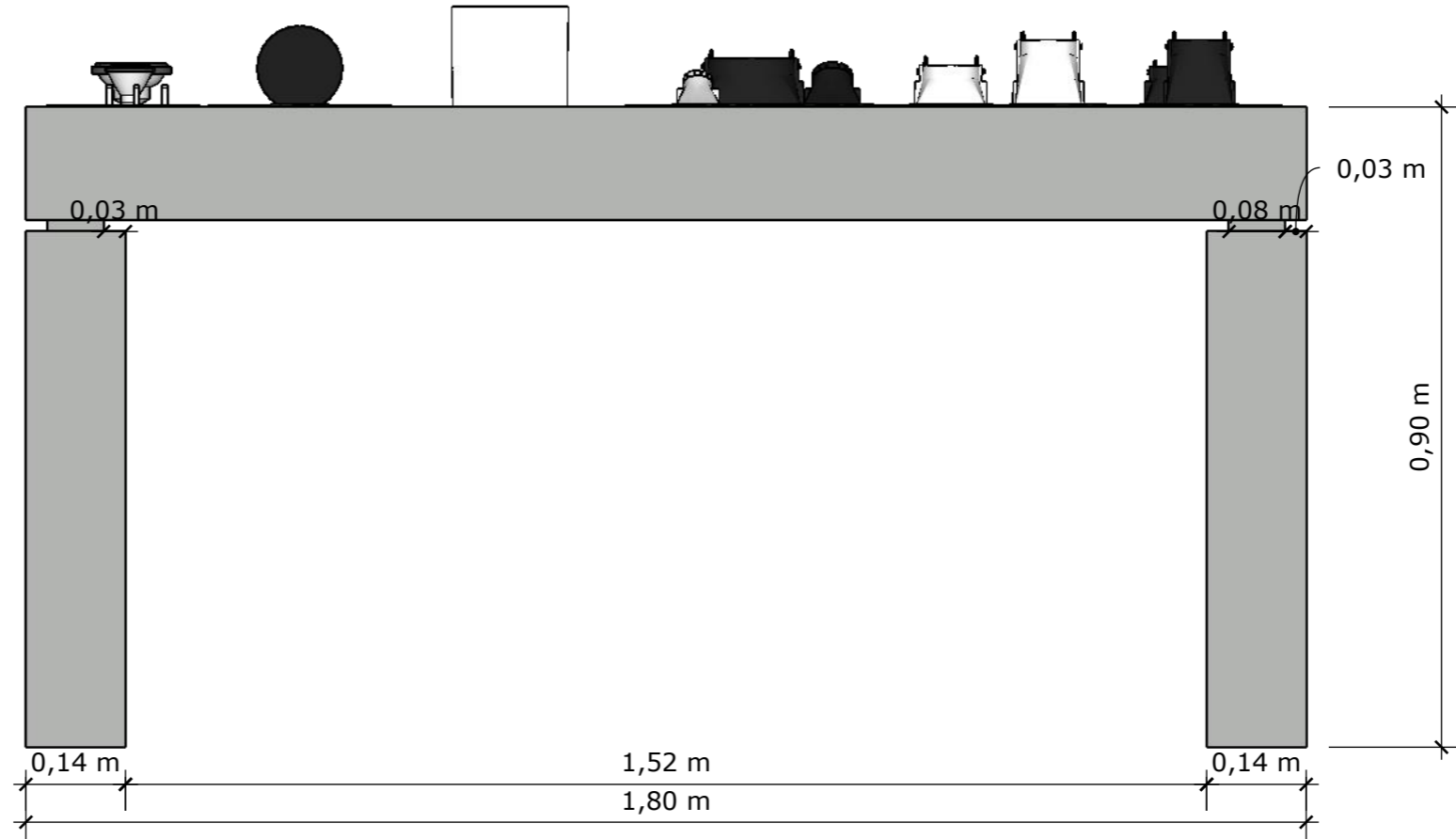
SIDE VIEW - SCALE 1/10
