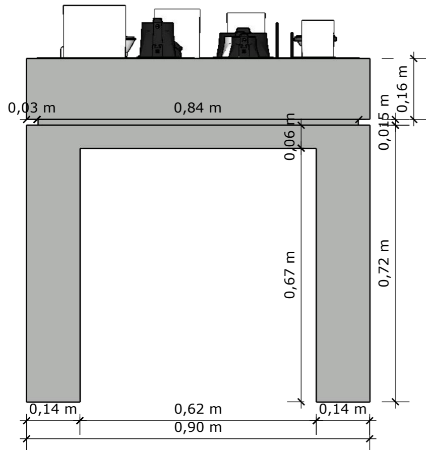
FRONT VIEW - SCALE 1/10
