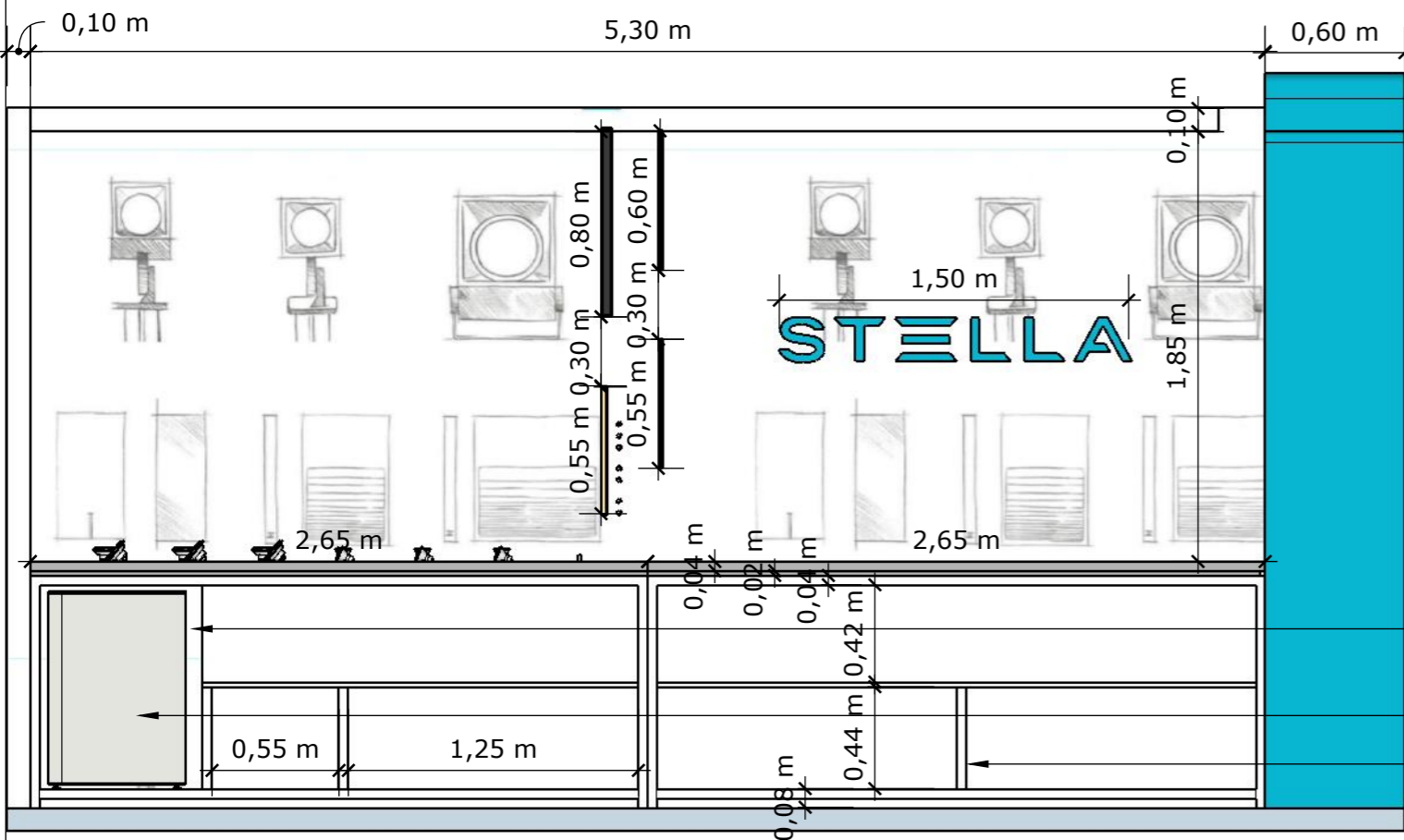
FRONT VIEW - SCALE 1/30
