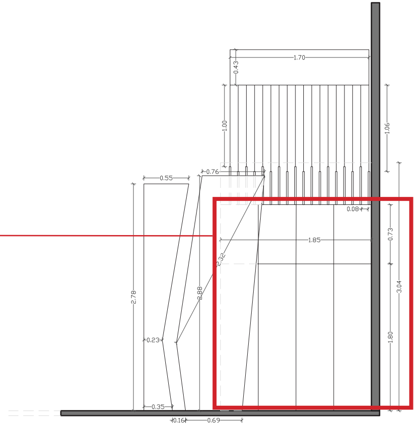
Meeting Dividers_elevation_right side view
