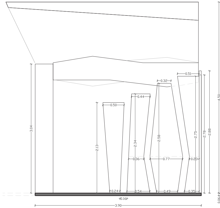
Meeting Dividers_elevation_front view
