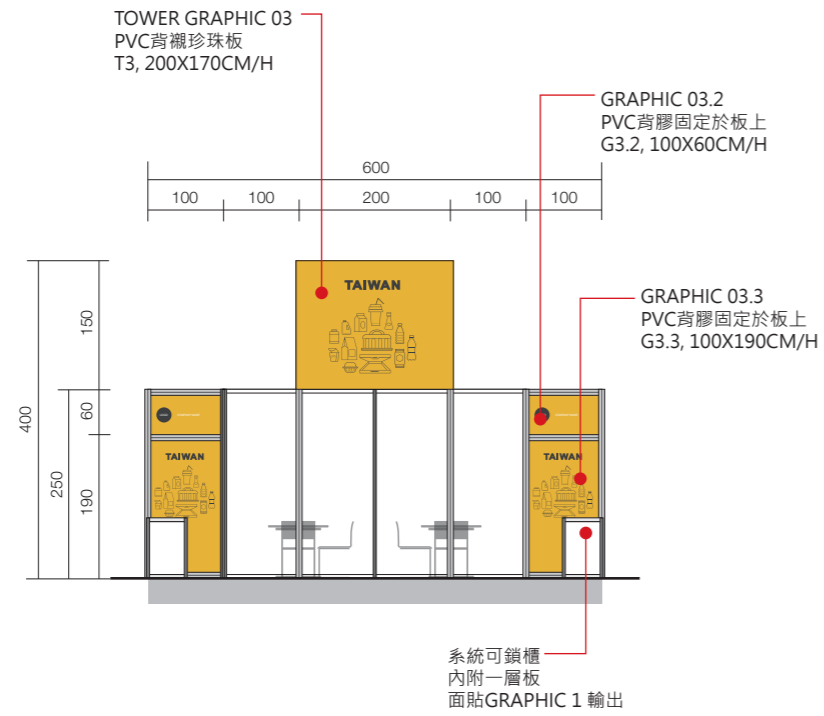
1 ELEVATION 11 1/100CM
