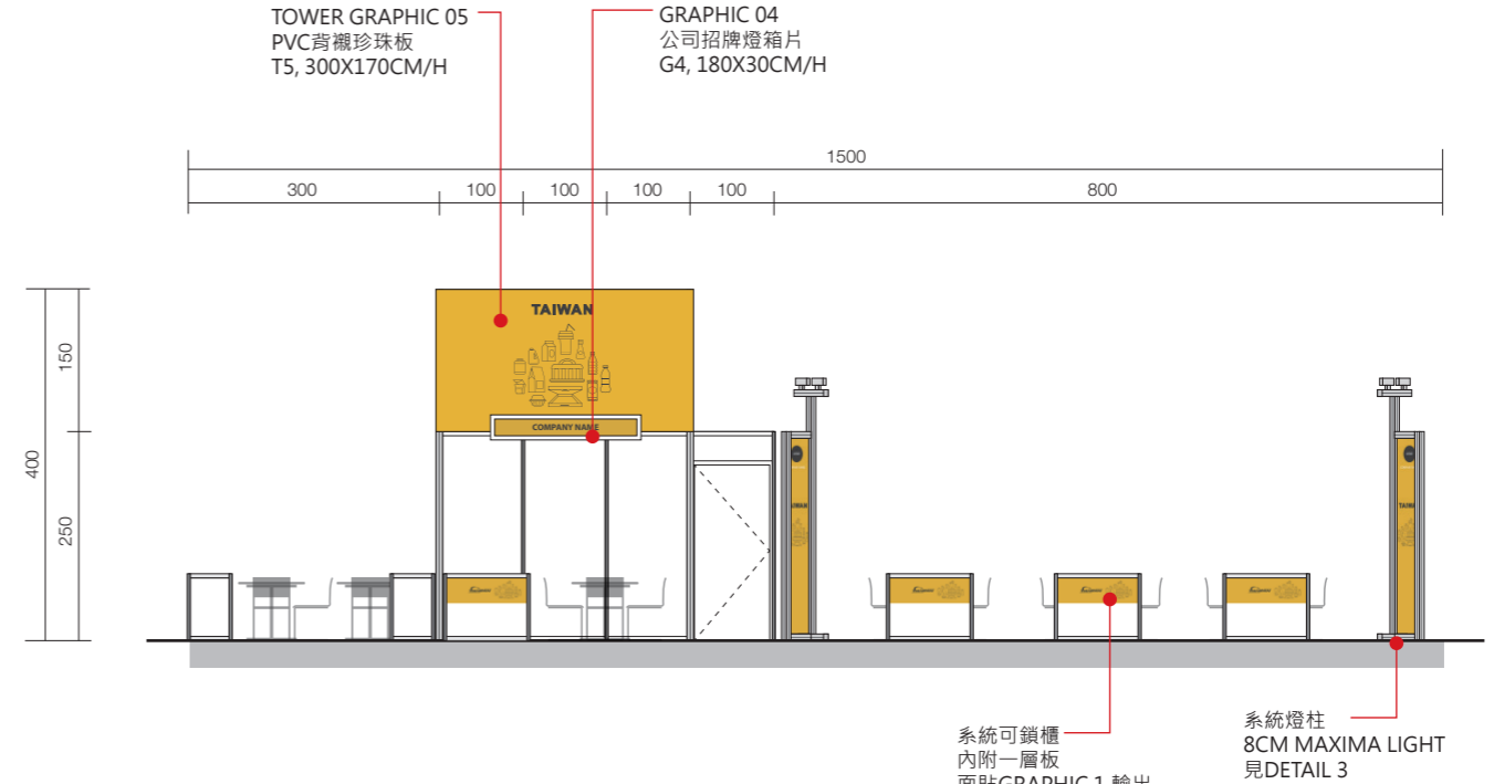
4 SECTION 10 1/100CM
